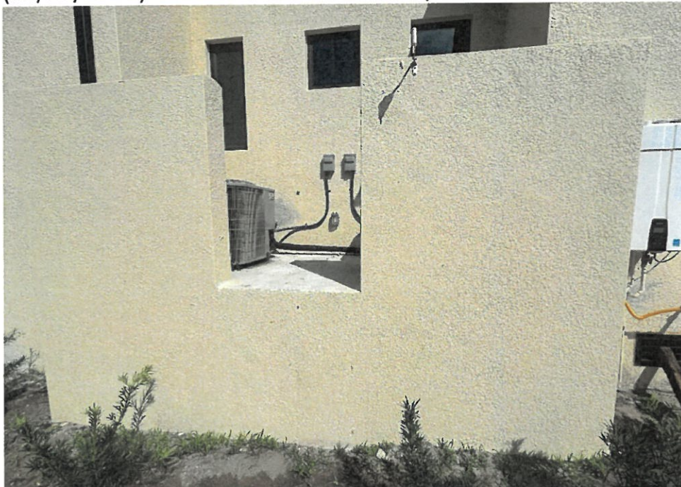
(05/27/2025) Elevated AC Enclosure Top of Slab=11.1'
