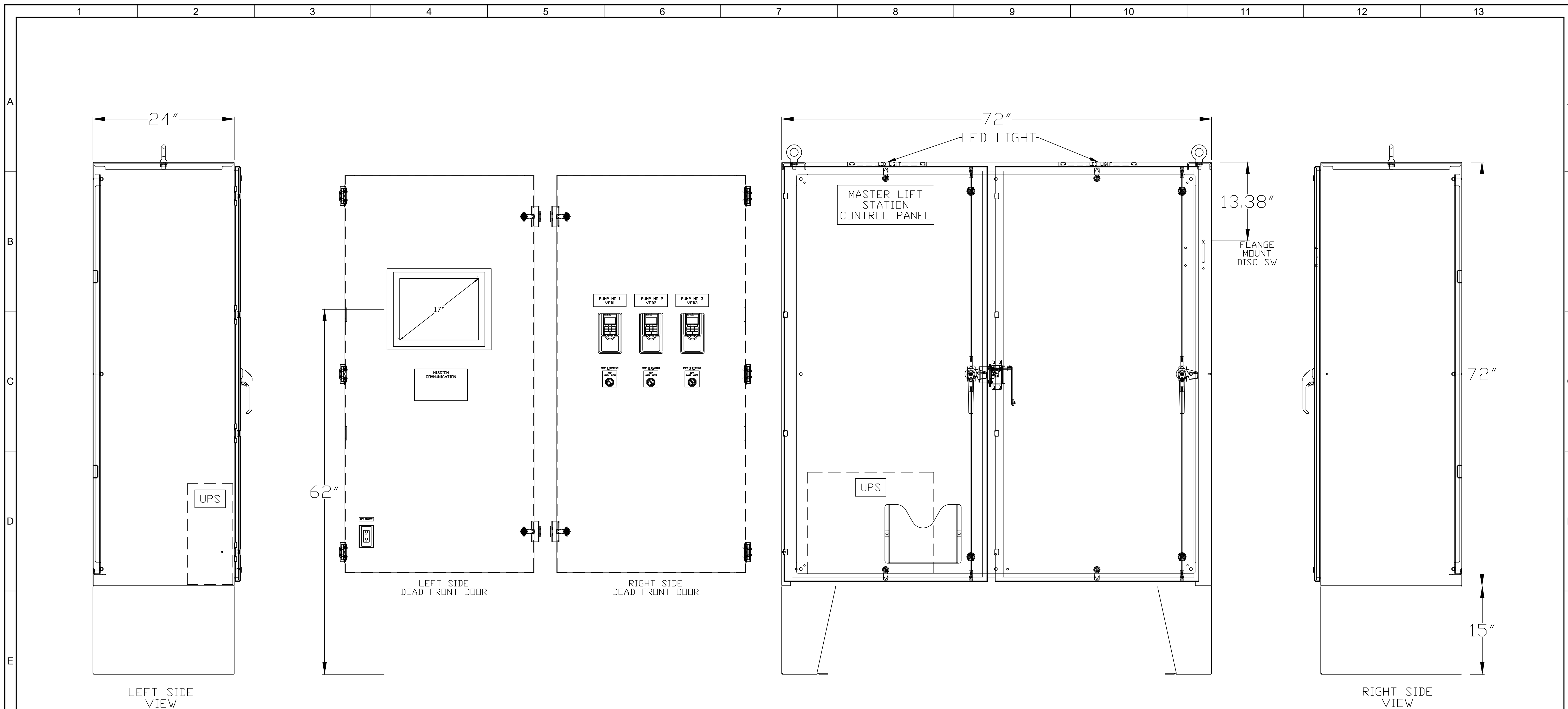
72"H X 72"W X 24"D ENCLOSURE, DISCONNECT TYPE, FLOOR MOUNT WITH 15" LEG KIT, TWO DOOR, CARBON STEEL. NEMA12, INNER DEAD FRONT DOOR FOR EACH OF THE TWO DOORS, MINIMUM OF 3" BACK FROM THE OUTER DOORS
