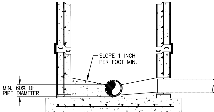
TYPICAL SECTION
