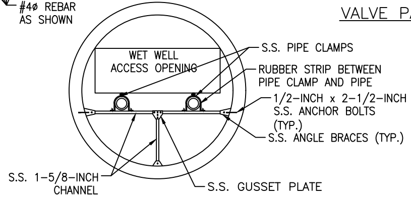
WET WELL PIPE BRACING DETAIL
